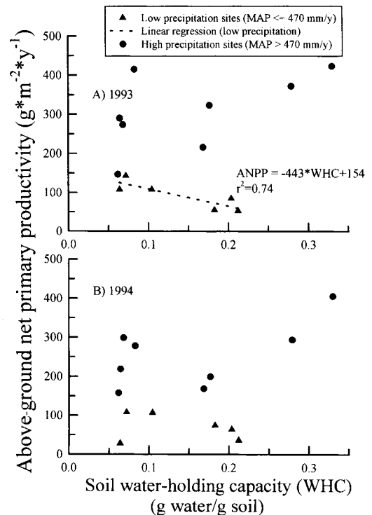
Fig. 3. Above-ground net primary productivity ( \text{g}\cdot\text{m}^{-2}\cdot\text{y}^{-1} ) in (A) 1993 and (B) 1994 as a function of soil water-holding capacity, with sites grouped by precipitation. Low precipitation sites have mean annual precipitation (MAP) less than or equal to 470 mm/y. High precipitation sites have MAP greater than 470 mm/y. Regression line and equation presented for the only significant linear regression.
