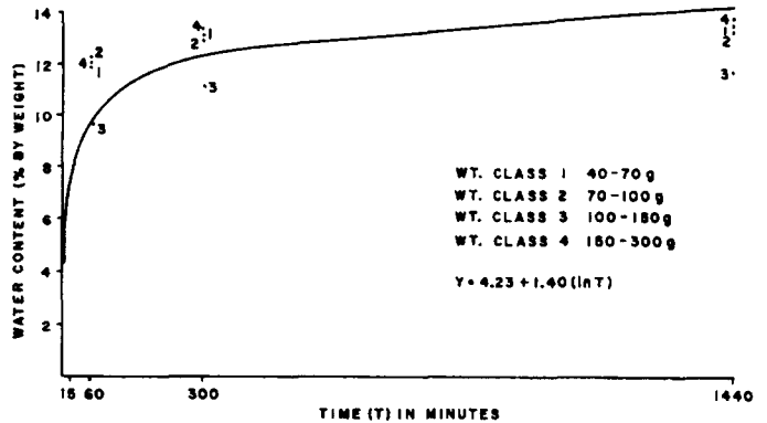
Fig. 1. Absorption curve of mean water content (% by weight) over time of 20 caliche rocks (all weight classes combined) submersed in water. Observed values at 60, 300, and 1440 minutes are shown for each weight class. The absorption curves of the different weight classes did not differ significantly ( P > 0.05 ).
