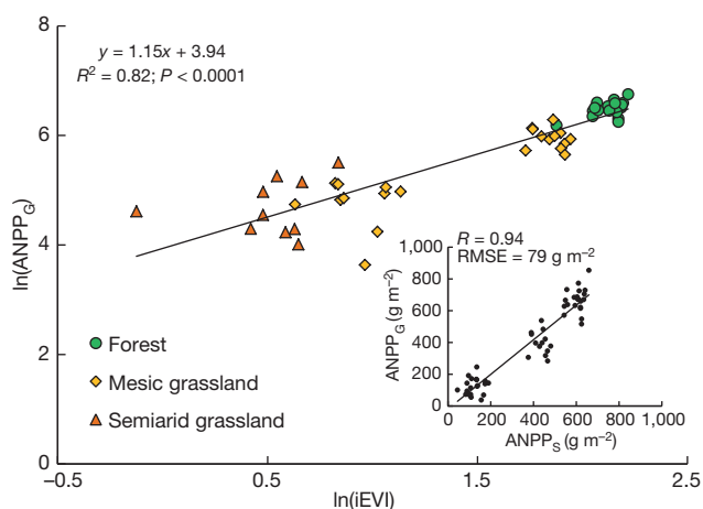
Figure 1 | Relationship between ANPP and iEVI. Relationship between in situ estimates of above-ground net primary production (ANPP G ) and iEVI derived from MODIS data (2000–2009) for ten sites across several biomes (see Supplementary Information and Supplementary Table 2). The solid line represents the linear regression used to estimate ANPP from iEVI (ANPP S ), in which \text{ANPP}_S = 51.42 \times \text{iEVI}^{1.15} . The inset shows the correlation between estimates of ANPP S and ANPP G for the ten sites over several years.
