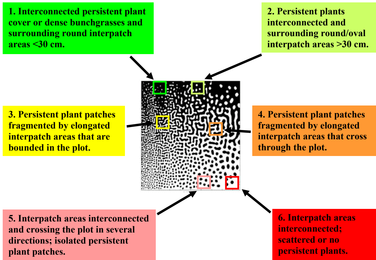
Figure 16. A schematic overview of resource retention classes (RRC) comparing the patterns described by each class. The image shows a continuum of patterns of vegetation fragmentation produced by a simulation model, where the dark areas represent persistent plant patches and the white areas are interpatch areas. The colored squares represent plots and the patch-interpatch patterns within each plot correspond to the associated RRC class. The figure was adapted from Rietkerk et al. (2004).
