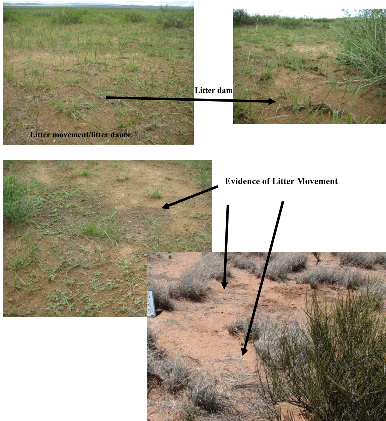
Figure A1. Litter movement is evidence of resource redistribution (transportation of litter from under plant canopies to plant interspaces by wind or water). As water flow increases it becomes sufficiently high to entrap larger and greater pieces of litter. Once water reaches an obstacle that slows or stops flow, litter is deposited behind these obstacles as litter dams. When soil is entrained within litter, there is evidence of soil redistribution.
