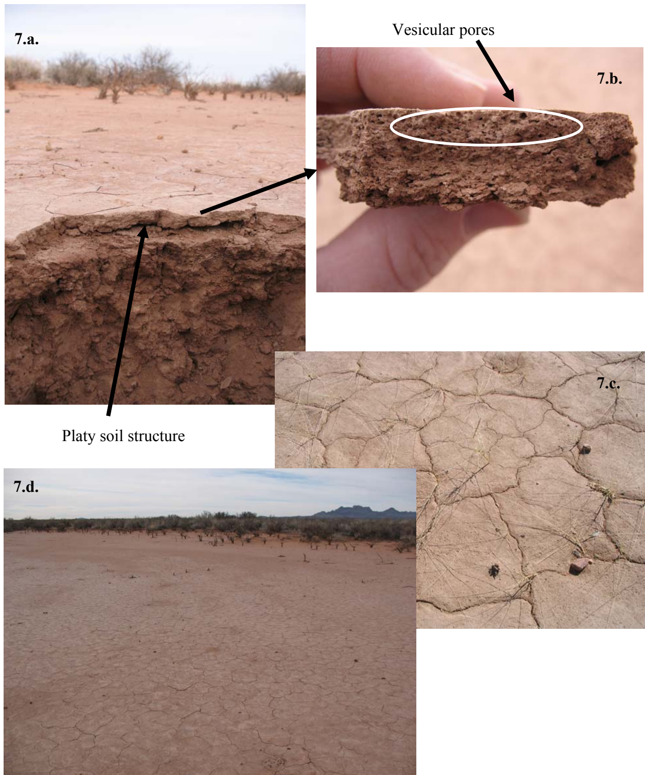
Figure 7. SP - Strong physical crust; usually platy or massive, no substantial biological component (Fig. 7.a.-d.). In some cases, biological or weak physical crusts can form on top of thick strong physical crusts. Thus, care should be taken to ensure that the entire pedoderm is observed by digging and lifting out surface peds that can be over 2 cm thick (Fig. 7.a.-b.). Vesicular pores can be present (Fig. 7.b.).
