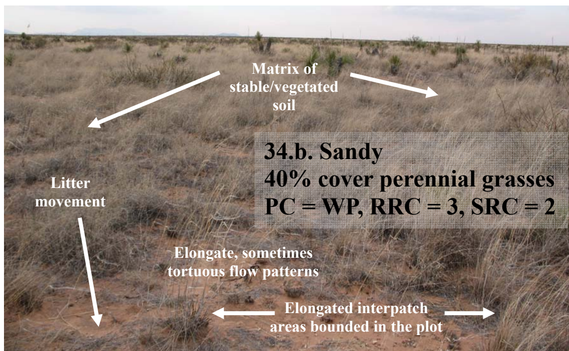
Figure 34. Both plots are in Sandy ecological sites and dominated by perennial grasses. The pedoderm (poorly developed biological crust), the small interpatches, and the stable soil (SRC = 0) of 34.a. convey that this plot has a higher potential for plant establishment, growth and survival as well as retaining soil and site resources compared to that of 34.b. The weak physical or biological crust coupled with the larger interpatches of 34.b. suggest a reduced resistance to wind and water erosion and disturbance (physical or introduction of weedy/invasive species). The SRC of 2 in 34.b. indicates reduced soil stability of the site. The site in 34.b. would be considered at greater risk of soil erosion and subsequent grass loss when compared to 34.a.
