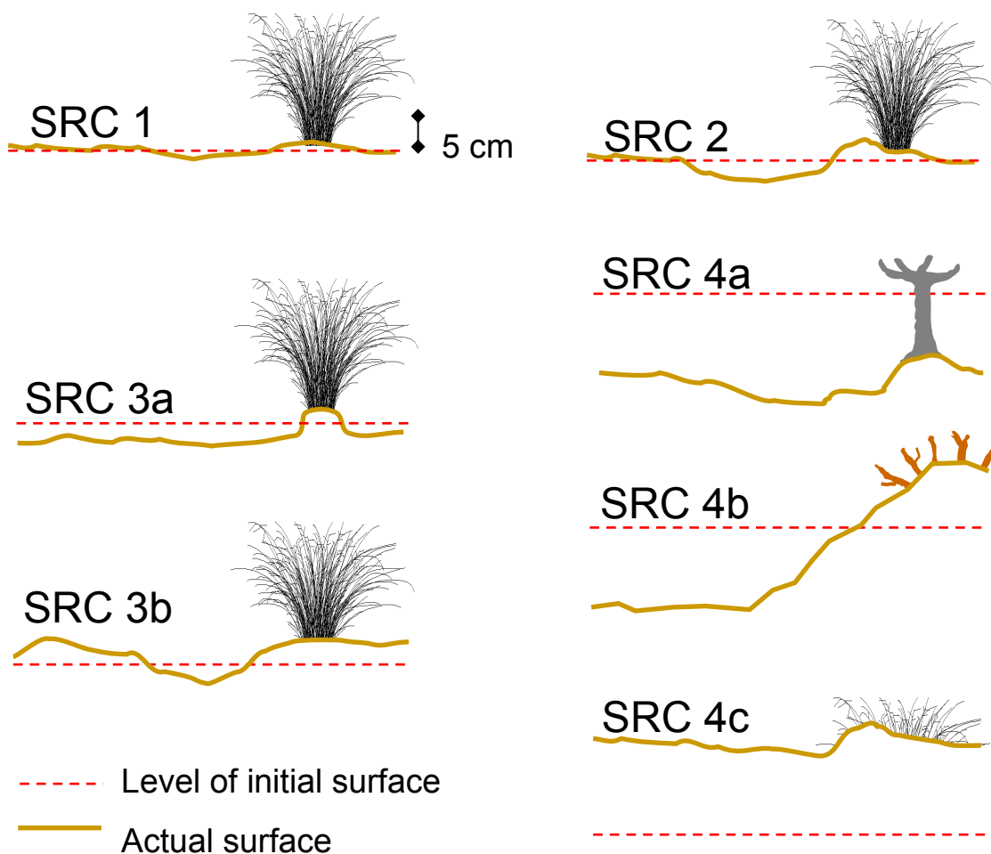
Figure 25. Depiction of increasing severity of soil redistribution with greater soil redistribution classes. Lateral extent of soil redistribution increases at higher classes.
