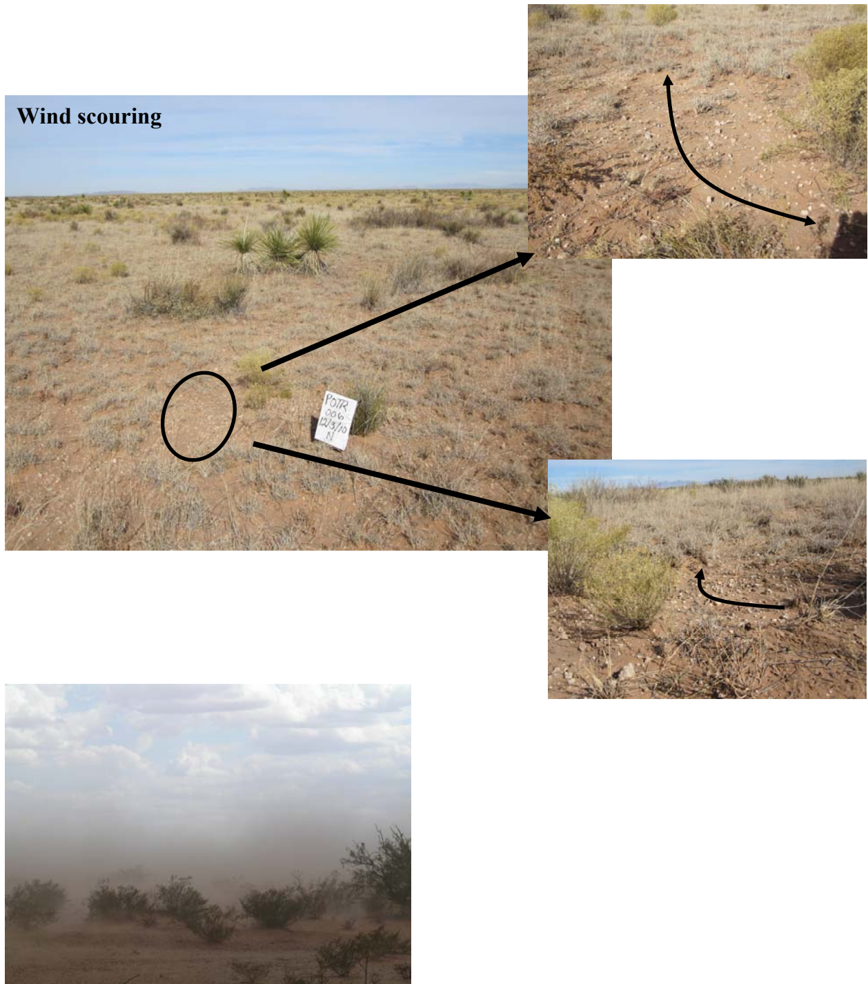
Figure A4. Wind erosion: wind scouring occurs when wind erosion removes finer soil particles from plant interspaces, forming elongated and slightly concaved depressions.
