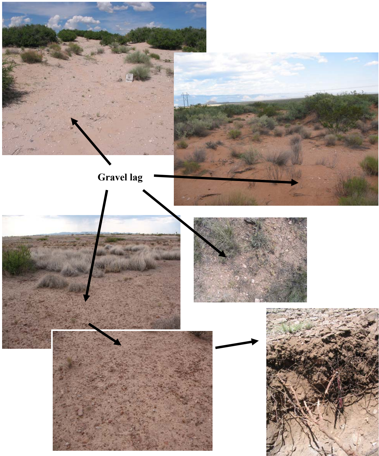
Figure A7. Wind and water erosion: A gravel lag is formed as rock fragments accumulate and remain at the soil surface after the removal of finer soil particles by wind or water erosion.
