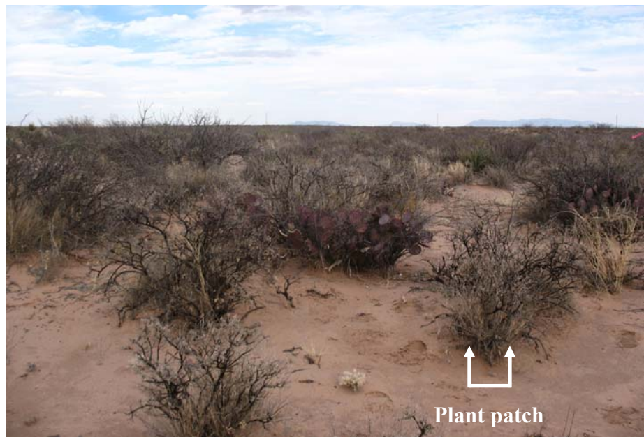
Figure 18. Plant patches here always include tarbush ( Flourensia cernua ; FLCE) accompanied by one or more additional species, almost always including a long-lived perennial mid-grass species. These plant patches can be described on the data form (Table 2) as FLCE mixed with perennial grasses and other species (SH w/ mid PG, etc). The width of a patch is shown with white arrows. Note that the patch width is smaller than the width of the canopy.
