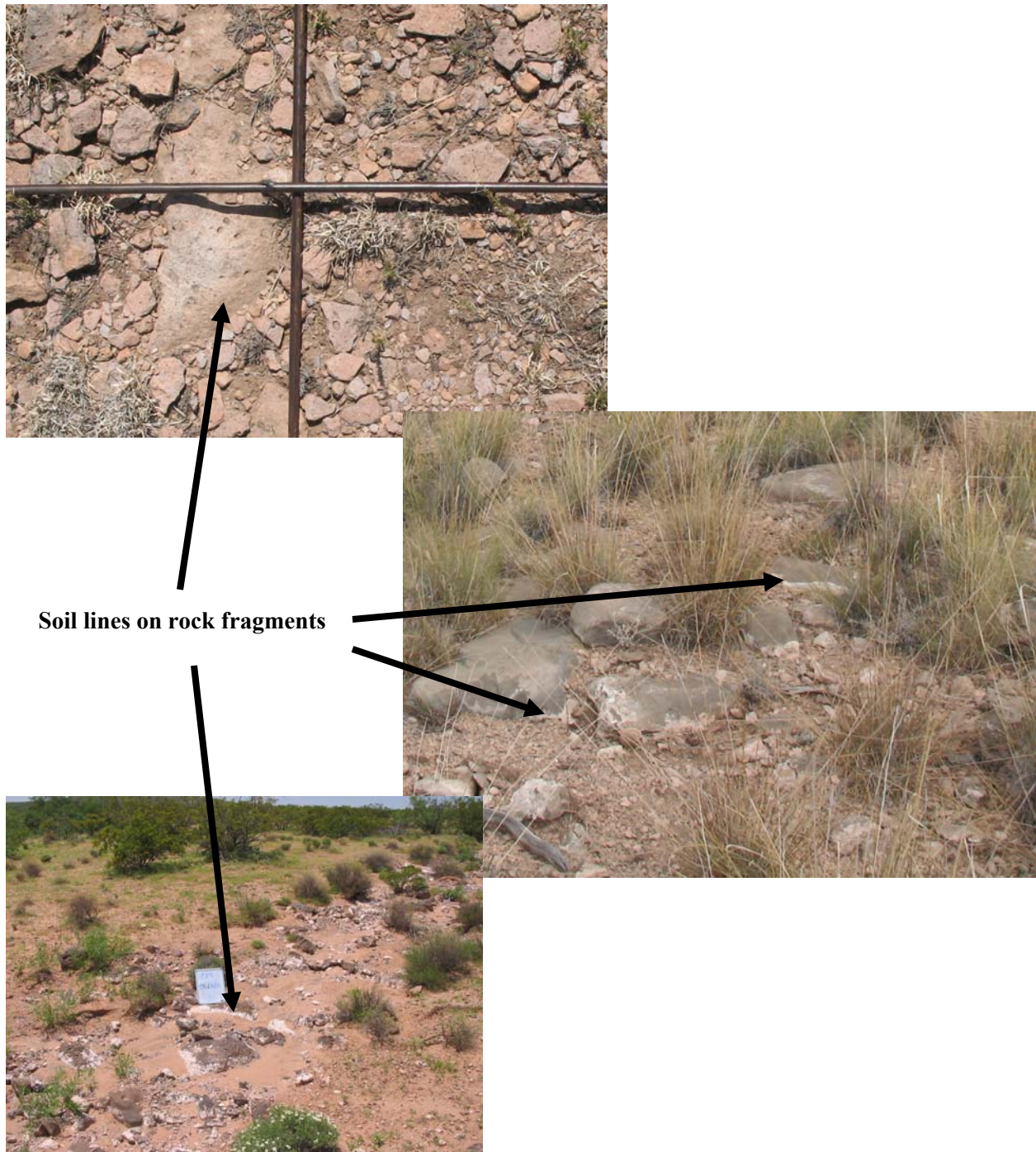
Figure A8. Wind and water erosion: soil lines on rock fragments appear as coatings of clay, carbonates, or silica, or mineral stains on the underside and sides of rock fragments. These features originally formed during pedogenesis and appear as a line or boundary around individual rock fragments where soil erodes from around rocks situated within the soil profile. Lines are roughly parallel to the soil surface unless the rock has been displaced. Clay coatings, carbonates, and silica are formed in B horizons. Clay coatings and mineral stains are red to brown; carbonates and silica are whitish. Carbonate collars around rocks in A horizons (e.g., desert pavement; McFadden et al. 1998) are evidence of erosion only where exposed by soil loss; see also carbonate coats on rock fragments.
