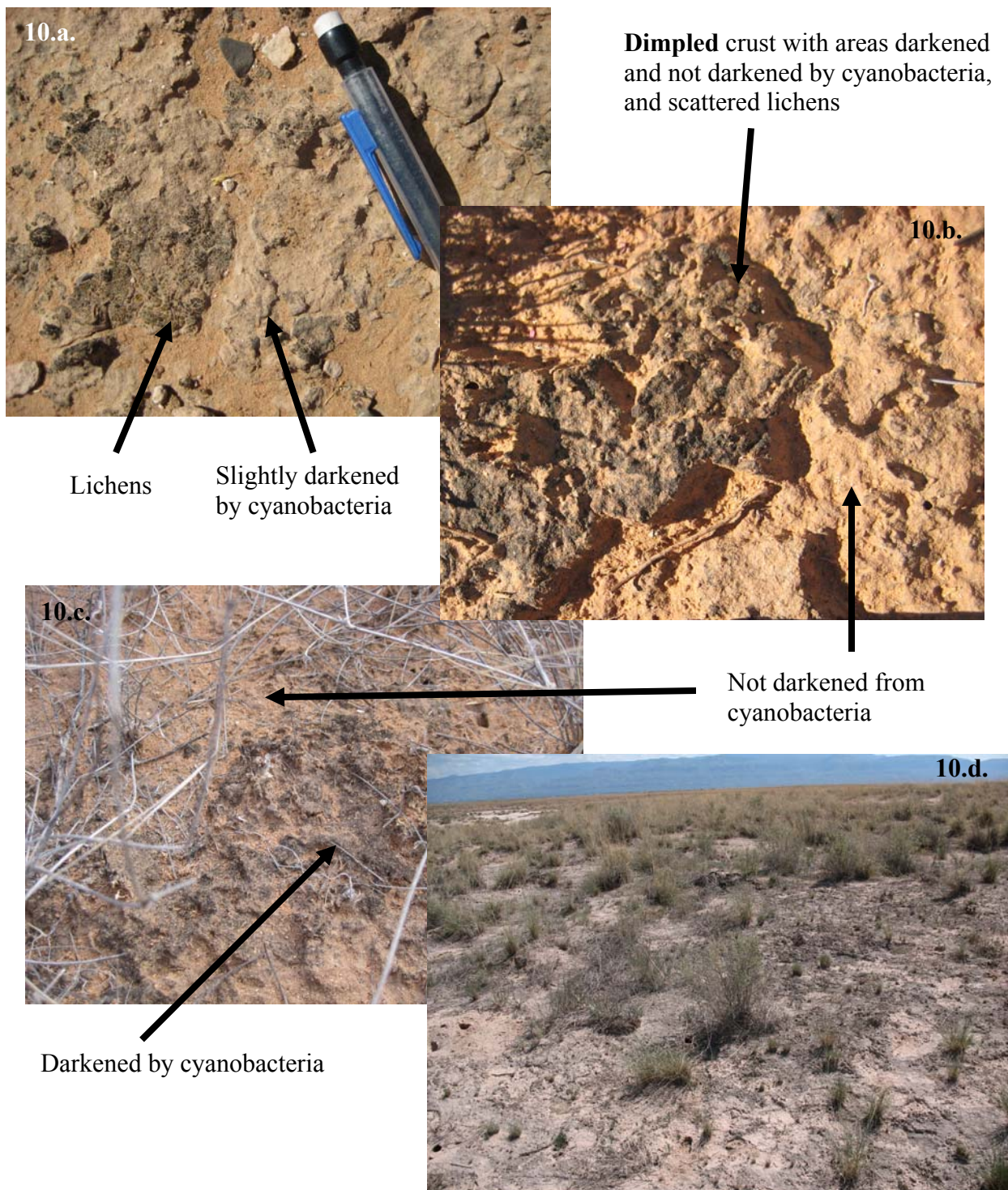
Figure 10. PDB - Poorly developed biological crust; discontinuous cover (broken or patchy) of one or more functional/structural group ( algae , lichen, moss or dense cyanobacteria) forms a smooth or dimpled crust, typically with \leq 1 cm of vertical relief (not rugose, rolling or pinnated; Fig. 10.a.). Poorly developed biological crusts are recognized by either (1) the dense cyanobacterial sheaths (Fig. 10.a.-d.) compared to weak physical or biological crusts, or (2) a discontinuous cover of one or more biological crust functional/structural group forming a smooth or dimpled crust (in contrast to the continuous, darkened rugose, rolling or pinnated crusts of the strongly developed biological crusts).
