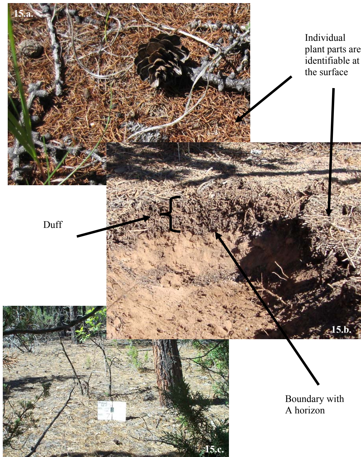
Figure 15. D - Duff; non-decomposed to fully decomposed plant and organic matter located above the A horizon (a patchy or continuous O horizon ). Individual leaves and plant parts are recognizable in the upper part of the duff layer, but become less discernable with depth (Fig. 15.a. & b.). Individual plant parts are not readily distinguished at the boundary with the A horizon (Fig. 15.b.).
