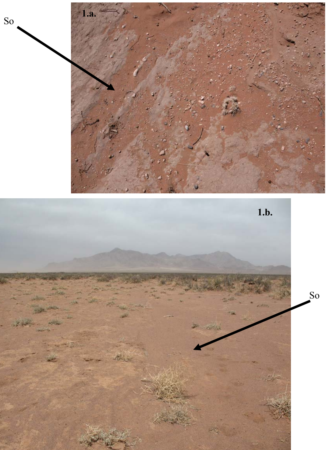
Figure 1. So - Loose soil over a pedoderm class. Arrows point to loose, structureless soil discontinuously covering the pedoderm. Note the difference in soil color between the loose soil (redder) and the soil it covers (grayer) in 1.a. In these examples, 'So' would be listed in the Pedoderm Class Modifier column to the far right of 'weak physical or biological crust' on the data form (the 'weak physical or biological crust' is the grayer soil in Fig. 1.a. and lighter/yellower soil in Fig. 1.b.).
