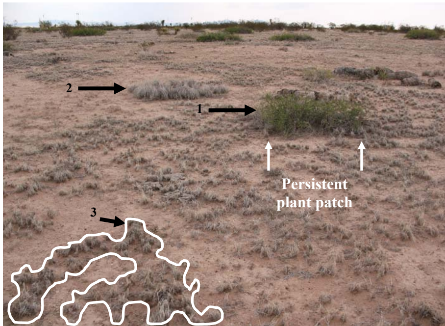
Figure 17. Three discrete patch types occur in this system. Patch composition is described on the data form (Table 2) by the plant codes (1) PRGL2 ( Prosopis glandulosa ), (2) PLMU3 ( Pleuraphis mutica ), and (3) SCBR2 ( Scleropogon brevifolius ; plant codes can be obtained at http://plants.usda.gov/java/ ). Or, patches can simply be described as (1) shrub, (2) perennial mid-grass and (3) perennial short grass. Codes can be used for lifeforms (e.g., SH, mid PG, short PG). The white arrows show the width of the PRGL2 patch. The white lines indicate the SCBR2 patch.
