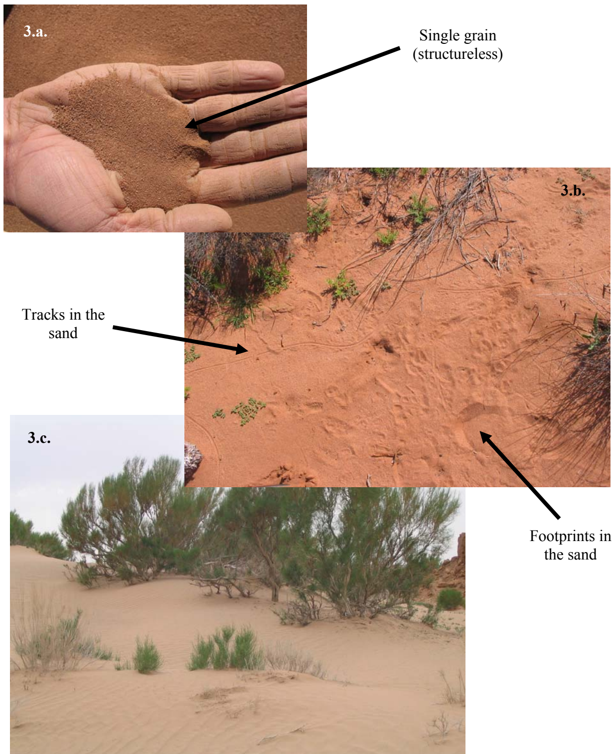
Figure 3. S - Bare single grain soil; pedoderm is characterized by bare mineral soil and no other class. Individual particles of soil less than 5 mm in diameter are visible in the hand (Fig. 3.a.). Animal tracks are frequently observed in a bare single grain soil pedoderm (left arrow of Fig 3.b.). The edges of human footprints look like tracks in sand and there are no structural aggregates broken up by footprints (bottom right arrow in Fig. 3.b.).
