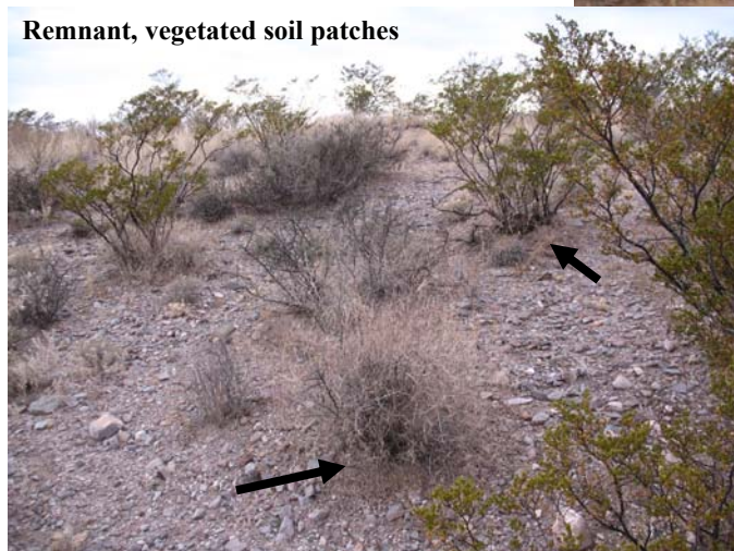
Figure A5. Soil mounds: these may be remnant, stable/vegetated soil patches (soil remaining in place after erosion, stabilized by persistent plant patches), depositional mounds (soil deposited at persistent plant patches that form obstacles to erosion and slow wind), or formed through a combination of erosion and deposition. To determine whether soil mounds indicate erosion, deposition or both, excavate to the persistent plant base and determine whether the plant base occurs above the non-mounded soil surface (evidence of erosion), below the soil surface (evidence of deposition), or above the non-mounded soil surface but below recent deposits (evidence of both). Recent soil deposits can appear as different-colored, loose or finely stratified soil.
