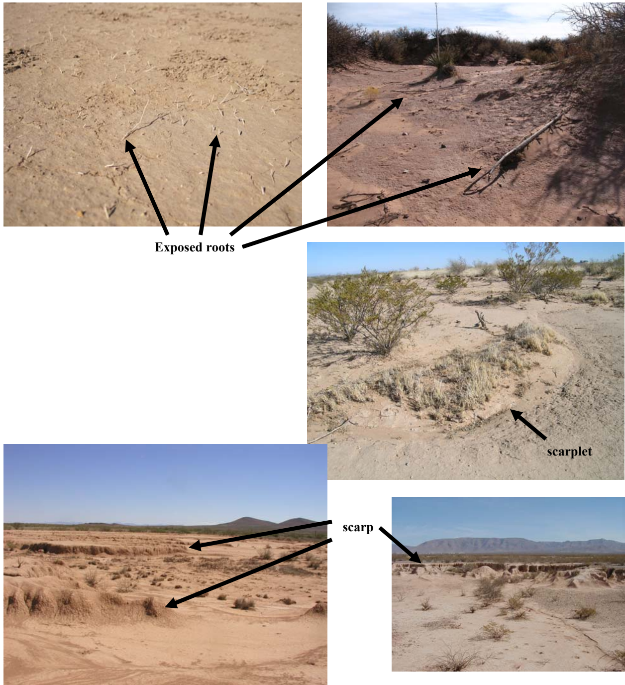
Figure A9. Wind and water erosion: exposed roots are a result of the thinning or loss of the soil surface. Vertical exposed roots include roots exposed below the plant base on plant pedestals and roots no longer attached to a plant stem or plant base (commonly seen as remnant grass roots). Vertical exposed roots indicate thinning of the surface horizon, at a minimum. Lateral exposed roots appear at the soil surface and typically occur with exposed subsoil/B horizon. A scarp is an escarpment, steep slope or structural bench of large (several meters or more) extent at the soil surface resulting from erosion; can be of any height, but typically less than 50 cm tall (adapted from SSSA 2008). A scarplet is a miniature scarp extending only a short distance laterally (no more than a few meters) and typically less than 20 cm tall.
